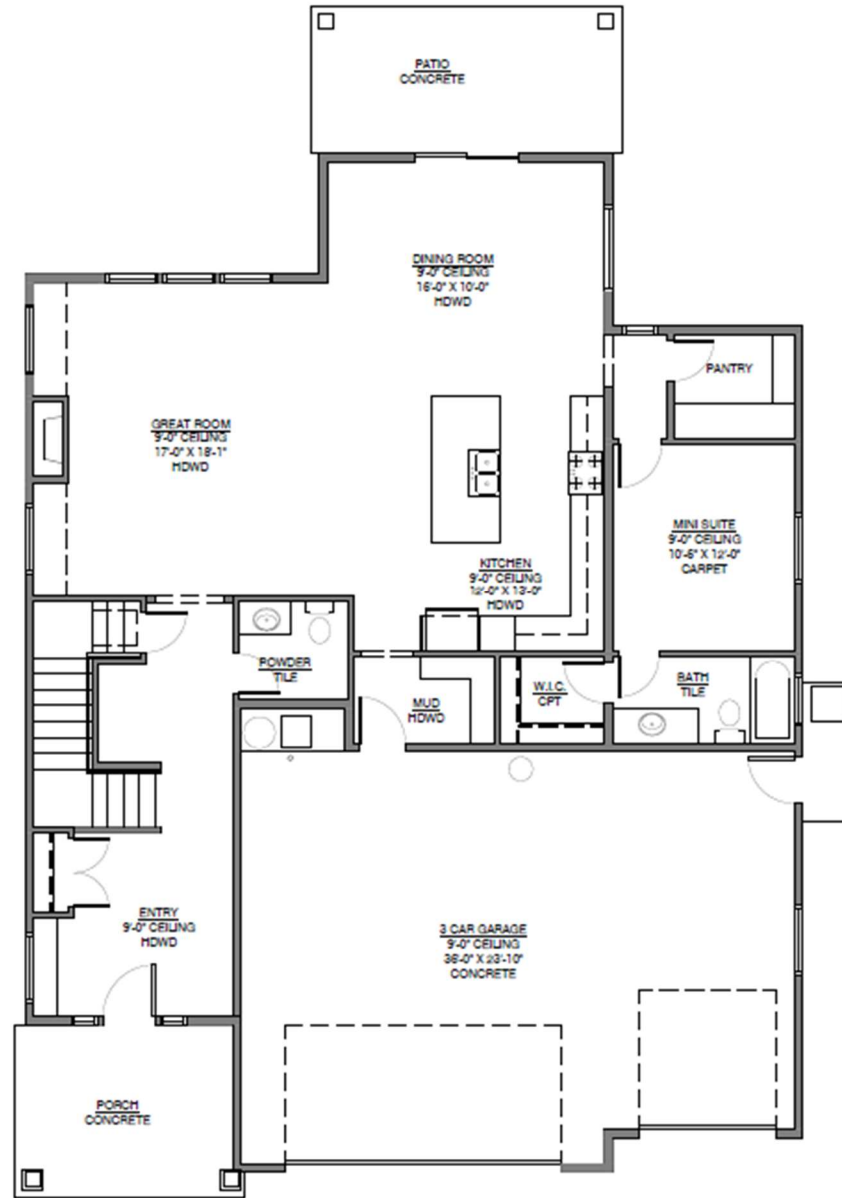
The Hailee- Main Floor
